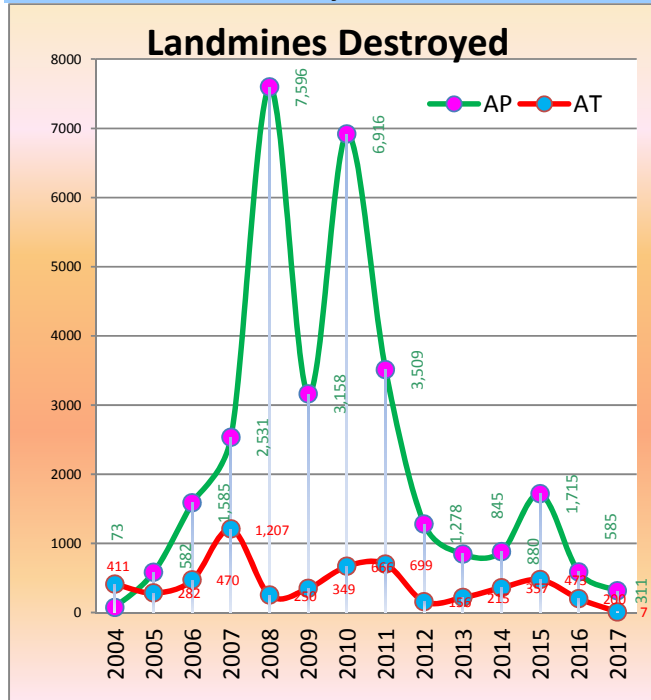
Chart 2.2: Devices Destroyed
