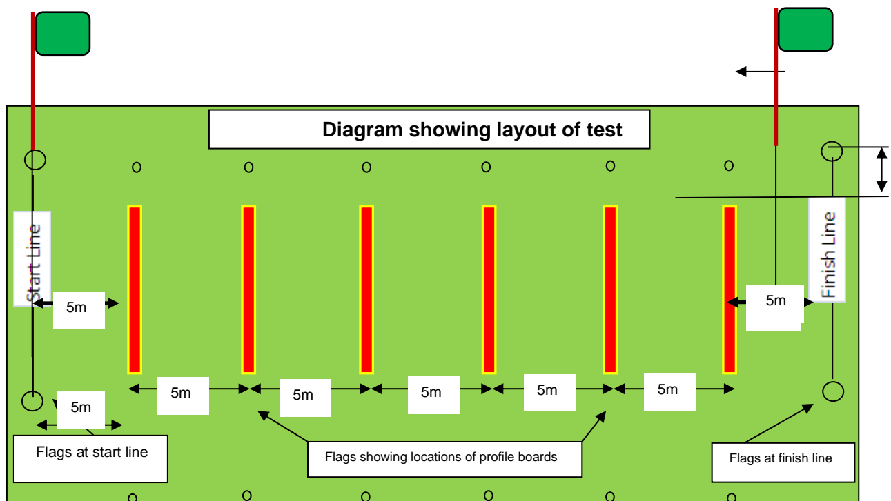
For comparison purposes, one extra profile board the same as the buried boards made of 3 – 6 mm chipboard or similar material should be placed on the ground outside the test strip.
